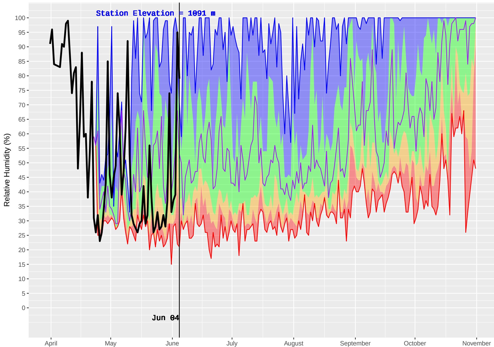
BIG MOUTH 2 (868) : Historical (2004–2016) and Current (2018) Noon Relative Humidity
