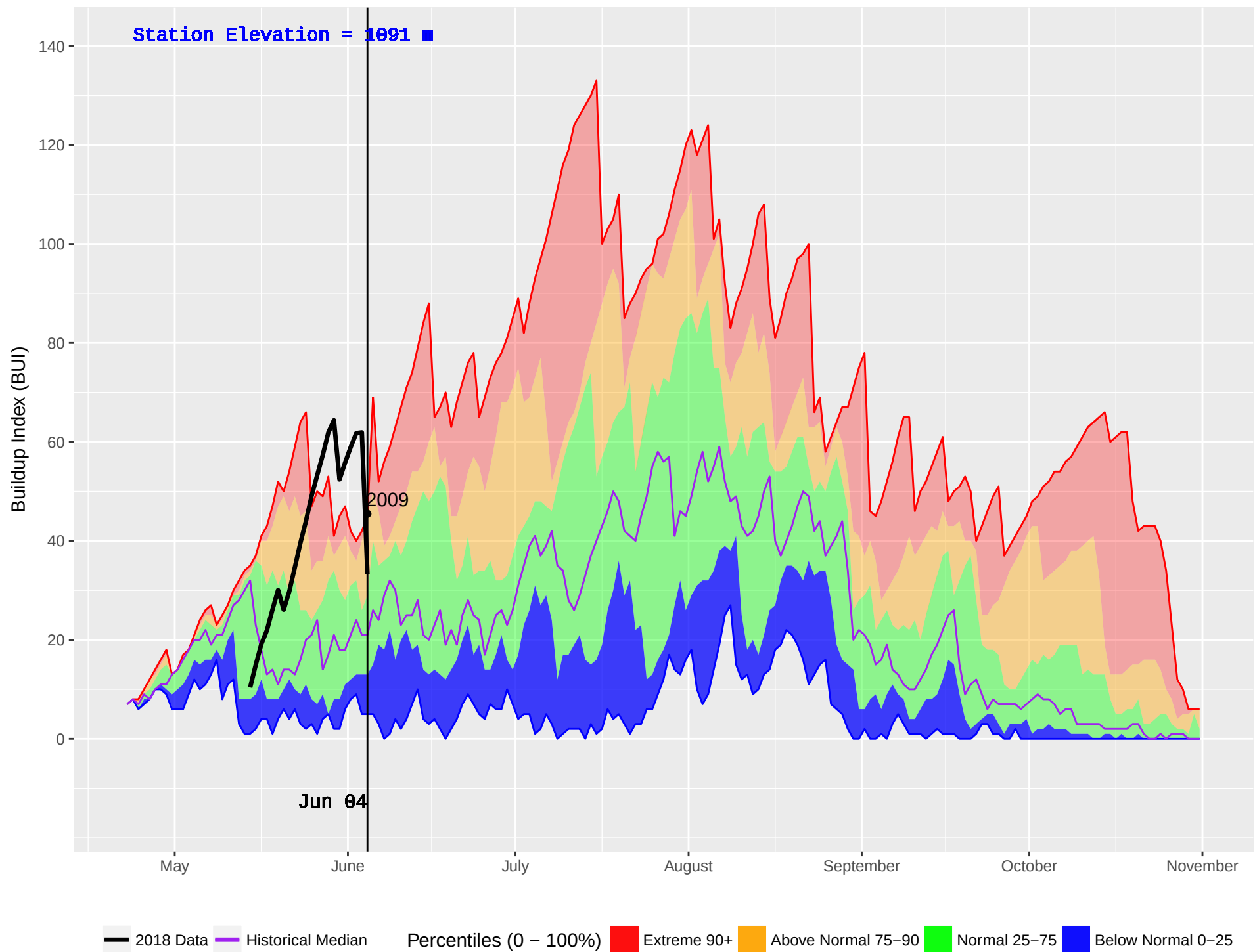
BIG MOUTH 2 (868) : Historical (2004–2016) and Current (2018) Noon Buildup Index (BUI)
